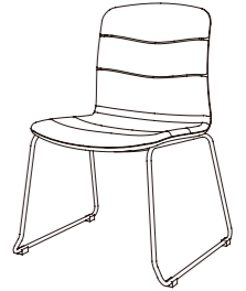
CRC11GM W565*D540*H780(mm)
