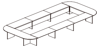
EU71-2 W5400*D2400*H760(mm)
