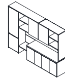
DL99(L/R)-2.19 W2560•D500• H1900
