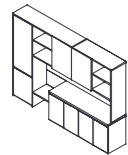
DL99(L/R)-2.19 W2560*D500*H1900
