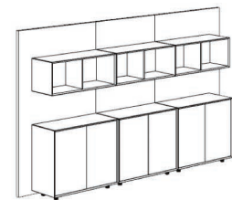
EI98 Filing Cabinet 3400(W)*490(D)*2000(H)
