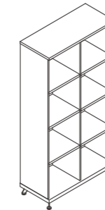
HM9H200 900Wx400Dx1805H
