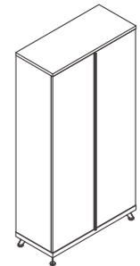
HM9H202 900Wx400Dx1805H
