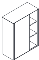
EY96.900 Cabinet W900*D400*H1150
