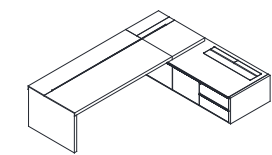
EY88.3000 Executive Desk W3000*D2200*H750
