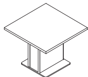
EY22.1800 Meeting Table W1000*D1000*H750
