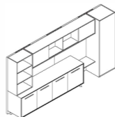
EA98(L/R) Cabinet W3600*D560*H1920
