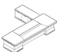
EX88 Executive Table W4060*D3120*H760 W3660*D3070*H760 W3260*D3070*H760
